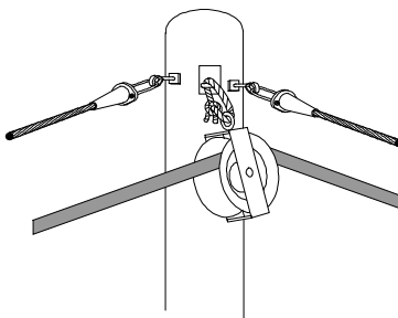
Figure 9 - Snatch block
