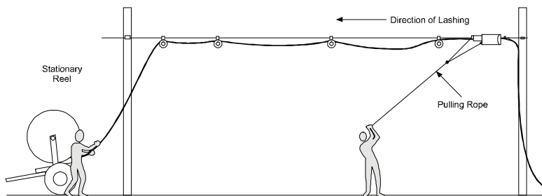
Figure 10 - Pull-back lashing of cable
